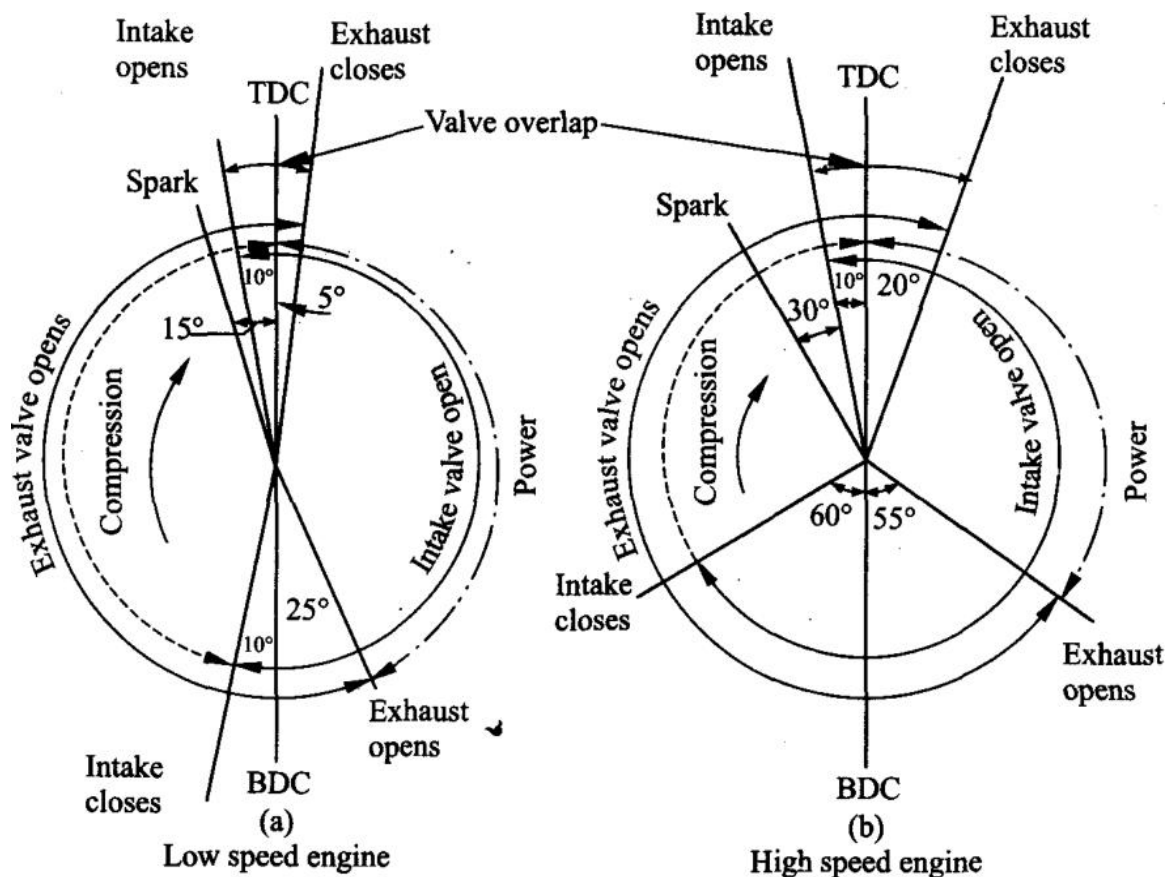
Fig. 1.11 Valve timing diagram for low and high speed 4-stroke SI engine
