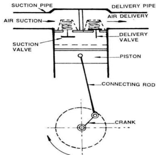
Fig : Single stage reciprocating Air Compressor
