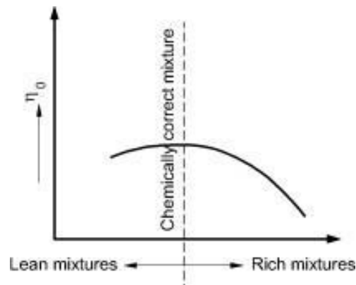
Fig. 9. 17 Brake thermal Vs Mixture strength
