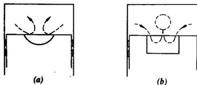
Fig.7. 23 Compression Swirl
