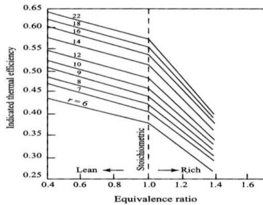
Fig. Effect of mixture strength on thermal efficiency for various compression ratios
