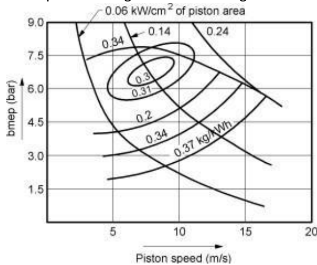
Fig. 9. 19 Performance map of a S.I. engine
