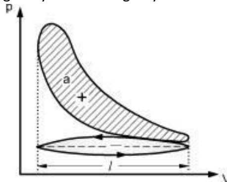
Fig. Indicator diagram
