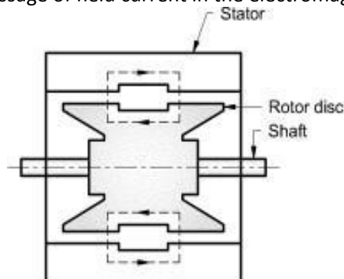
Fig. 9. 6 Eddy current dynamometer
