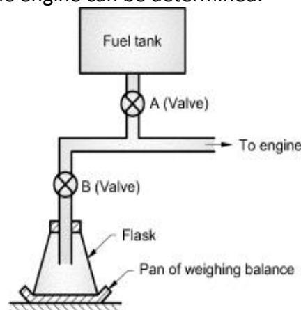
Fig. Direct weighing of fuel flow
