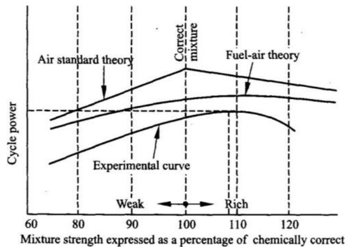
Fig. Effect of fuel-air ratio on power
