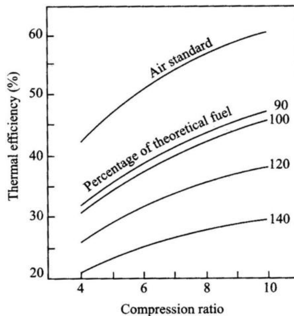
Fig. Effect of compression ratio and mixture strength on efficiency
