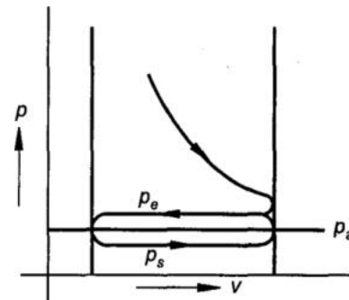
Fig. Pumping Loss
