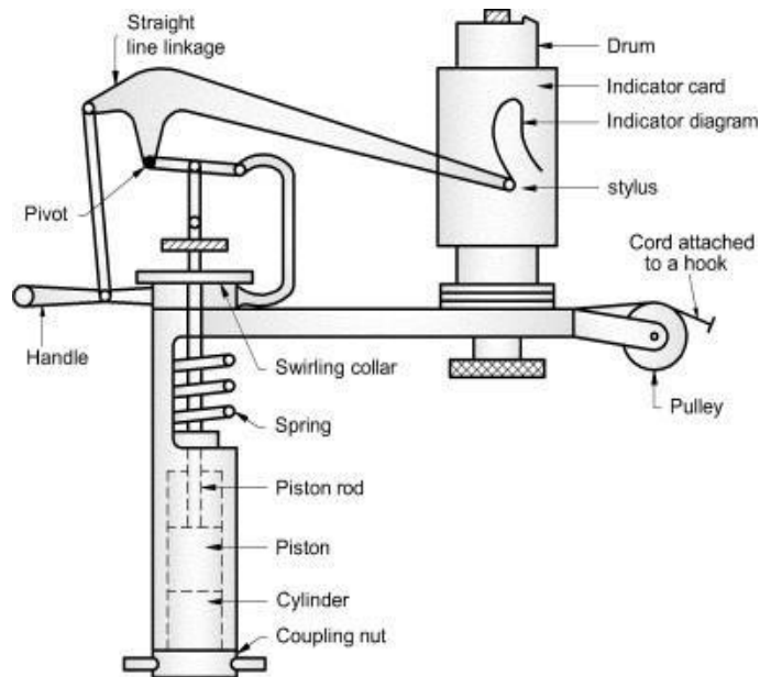
Fig. Engine indicator (Mechanical type)
