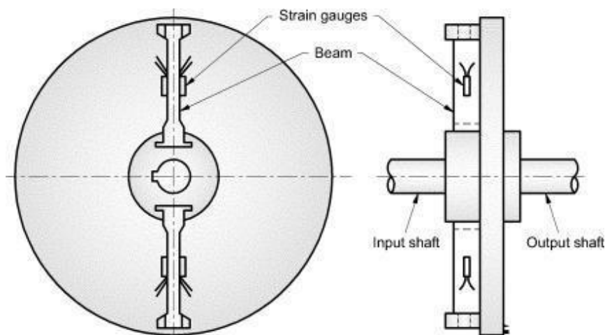
Fig. 9. 7 Transmission dynamometers
