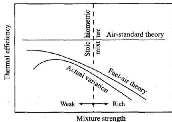
Fig. Effect of mixture strength on thermal efficiency
