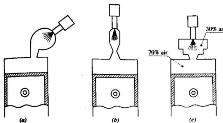
Fig. Pre combustion chamber
