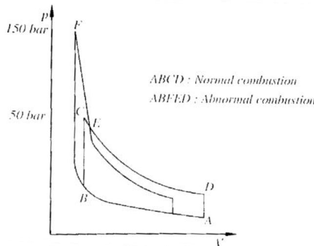
Fig.7. 10 Pressure rise due to knocking
