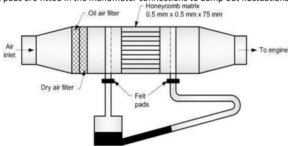
Fig. Alcock viscous air flow meter
