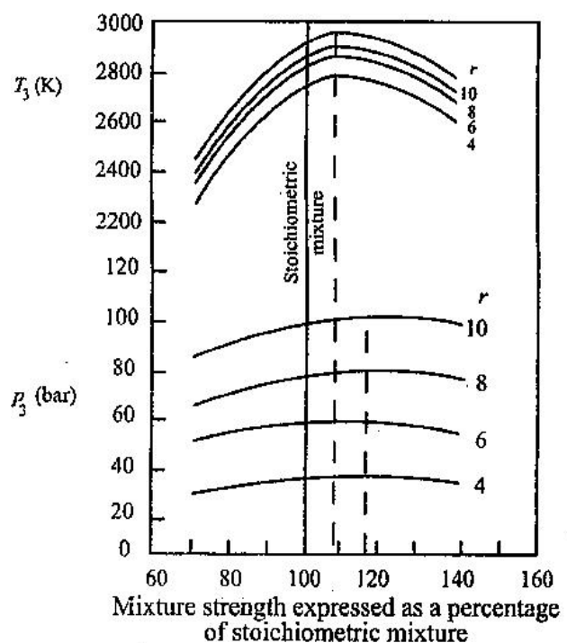
Fig. Effect of equivalence ratio on T_3 and P_3
