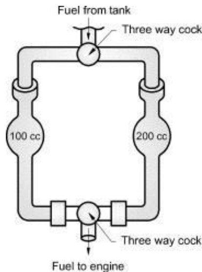
Fig. Volumetric Type Fuel Flow meter
