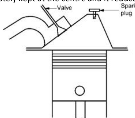
Fig.7. 16 Wedge head combustion chamber
