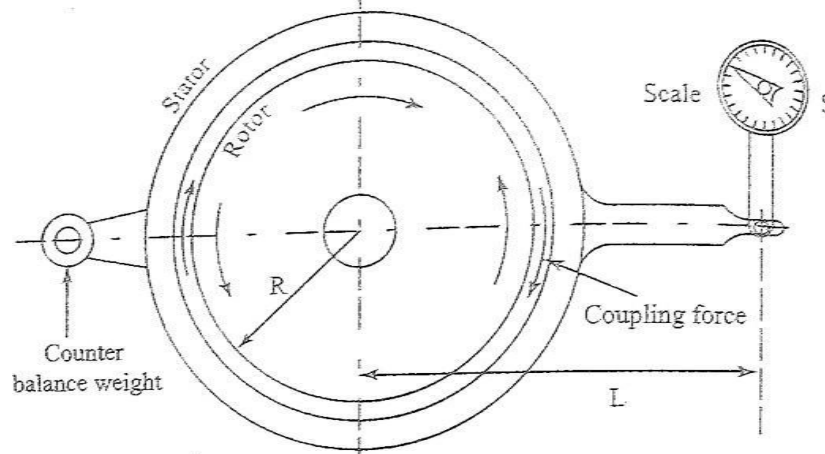
Fig. Principle of a dynamometer
