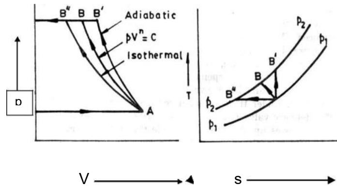
Fig: 4.3 Compression processes A-B'': Isothermal; A-B: Polytropic; A-B': Isentropic
