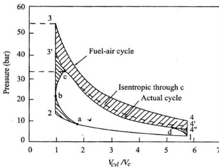
Fig. Effect of time losses on p-V diagram
