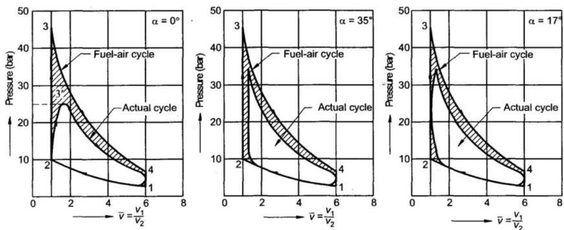
Fig. Effects of angle of advance \alpha on p-v diagram
