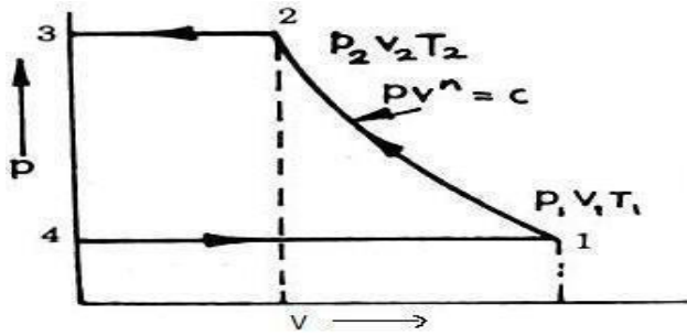
Fig: Polytropic compression (Compression follows pV = \text{Constant} )
