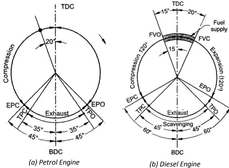
Fig.1.13 Port Timing Diagram for 2-stroke Engine
