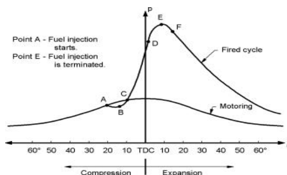
Fig. Combustion stages in C.I. Engines
