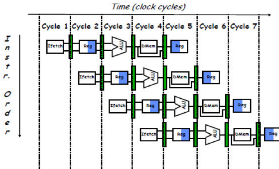
Figure 2.4 Pipeline activity
