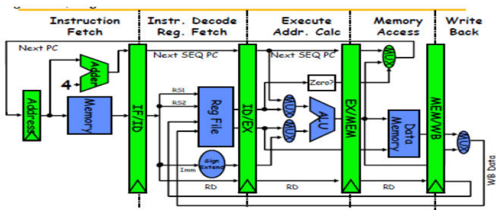
Figure 2.3 Functional units of 5 stage Pipeline. IF/ID is a buffer between IF and ID stage.
