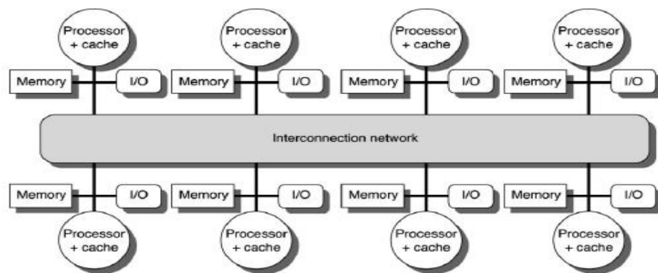
Distributed-memory multiprocessor
