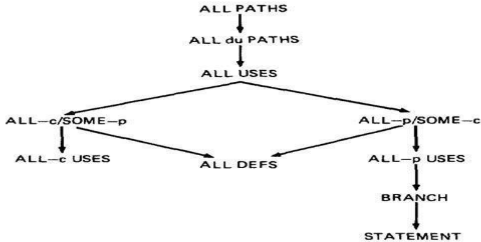
Figure 3.12: Relative Strength of Structural Test Strategies.
