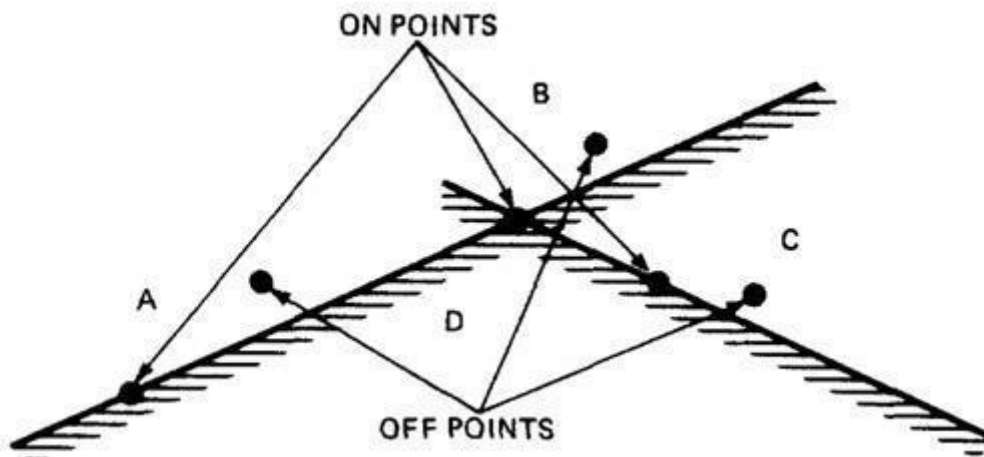
Figure 4.11: On points and Off points. ○ Figure 4.12 shows generic domain bugs: closure bug, shifted boundaries, tilted boundaries, extra boundary, missing boundary.
