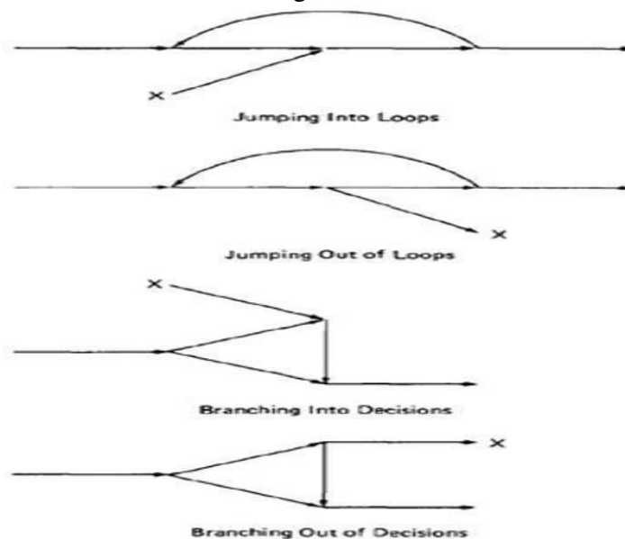
Figure 5.8: Un-structured sub-graphs.
