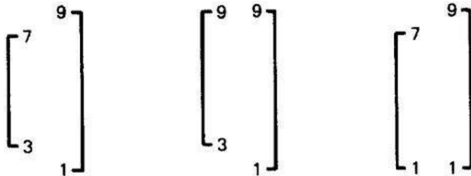
Figure 4.18: Harmless Range / Domain Span incompatibility bug (Caller Span is smaller than Called). ○ In all cases, the caller's range is a subset of the called's domain. That's not necessarily a bug. ○ The routine is used by many callers; some require values inside a range and some don't. This kind of span incompatibility is a bug only if the caller expects the called routine to validate the called number for the caller. ○ Figure 4.19a shows the opposite situation, in which the called routine's domain has a smaller span than the caller expects. All of these examples are buggy.
