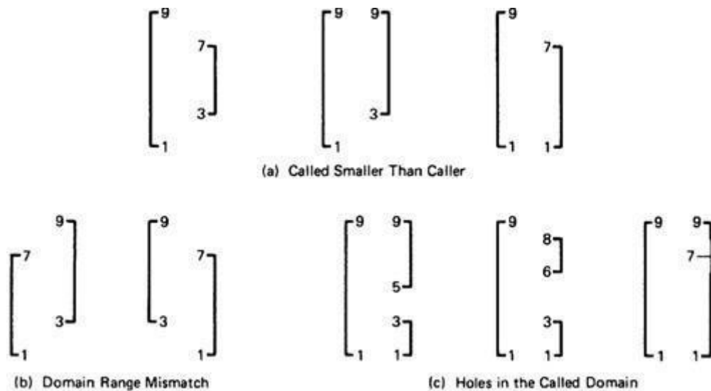
Figure 4.19: Buggy Range / Domain Mismatches ◦ In Figure 4.19b the ranges and domains don't line up; hence good values are rejected, bad values are accepted, and if the called routine isn't robust enough, we have crashes. ◦ Figure 4.19c combines these notions to show various ways we can have holes in the domain: these are all probably buggy.
