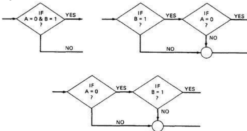
Figure 2.8: Alternative Flow graphs for same logic
