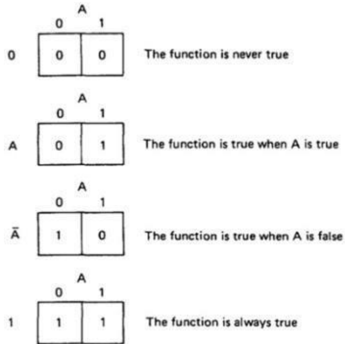
Figure 6.6 : KV Charts for Functions of a Single Variable. ○ The charts show all possible truth values that the variable A can have. ○ A "1" means the variable's value is "1" or TRUE. A "0" means that the variable's value is 0 or FALSE. ○ The entry in the box (0 or 1) specifies whether the function that the chart represents is true or false for that value of the variable. ○ We usually do not explicitly put in 0 entries but specify only the conditions under which the function is true.
