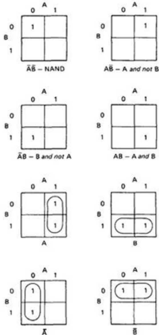
Figure 6.7: KV Charts for Functions of Two Variables. ○ Each box corresponds to the combination of values of the variables for the row and column of that box.
