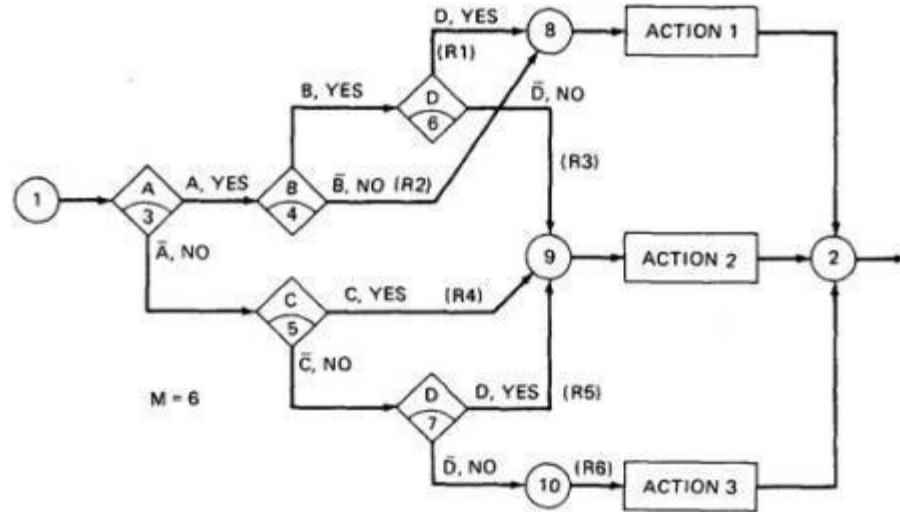
Figure 6.4 : A Sample Program ○ If the decision appears on a path, put in a YES or NO as appropriate. If the decision does not appear on the path, put in an I, Rule 1 does not contain decision C, therefore its entries are: YES, YES, I, YES.
