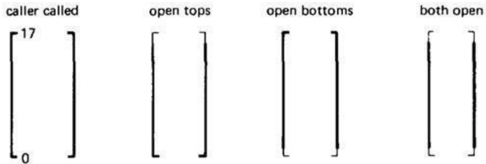
Figure 4.16: Range / Domain Closure Compatibility. ○ Figure 4.17 shows the twelve different ways the caller and the called can disagree about closure. Not all of them are necessarily bugs. The four cases in which a caller boundary is open and the called is closed (marked with a "?") are probably not buggy. It means that the caller will not supply such values but the called can accept them.
