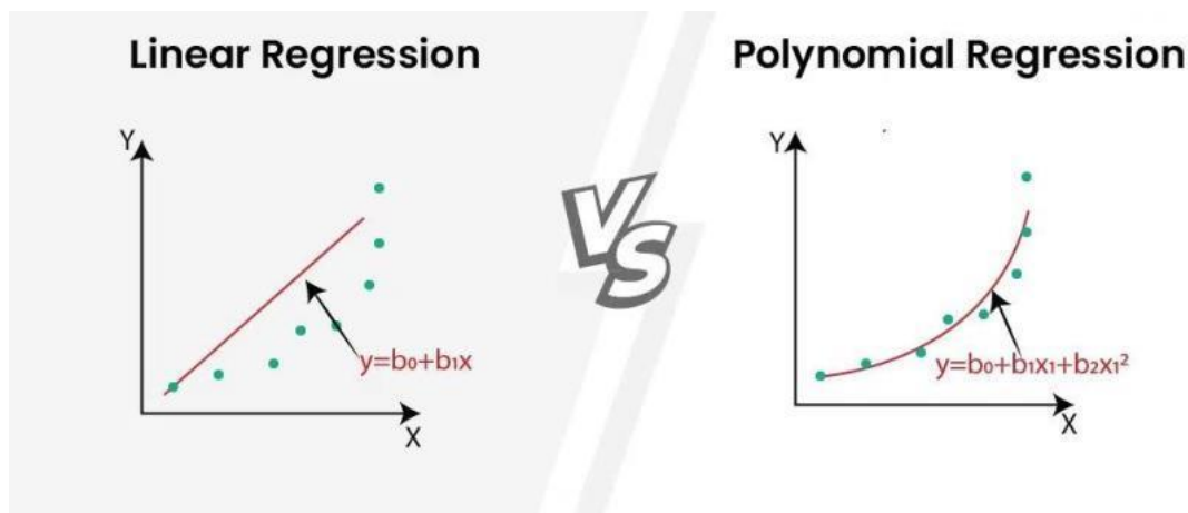
Linear Regression and Polynomial Regression
